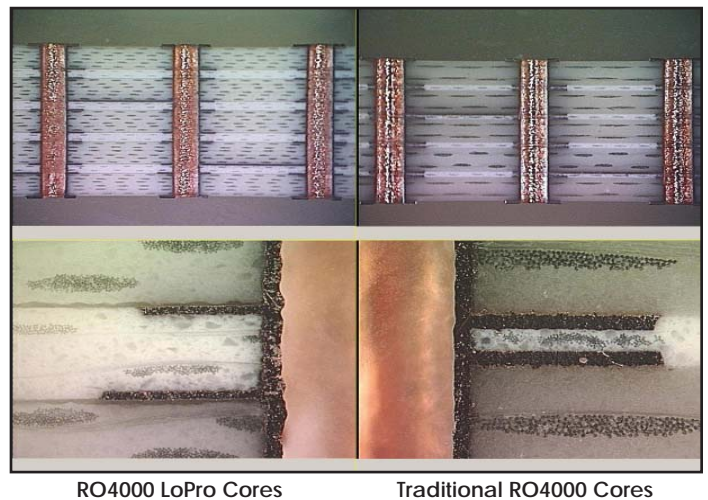
Visual comparison of RO4000 LoPro laminates and traditional RO4000 cores in multi-layer constructions.
