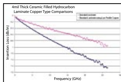
Fig 5 A Ceramic Filled Hydrocarbon Laminate Compared to the Same Laminate Using a Low Profile Copper and Showing Insertion Loss Over Frequency 2
