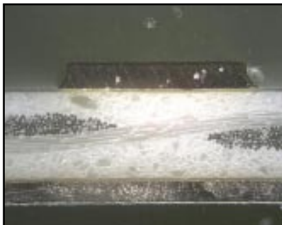
Fig 2 Example of Glass Weave on Microvariation of Dielectric Constant
