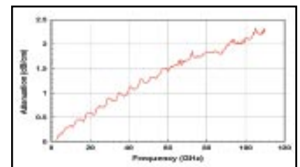
Fig 4 Attenuation Curve of CBCPW Using 2-mil. Thick LCP
