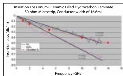
Fig 6 Data Showing Insertion Loss vs. Frequency of Copper Only as Compared to Copper Plated With ENIG (electroless nickel/immersion gold)
