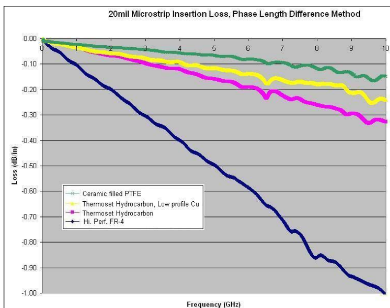
Figure 3 – The R04350B materials mentioned here are a thermoset hydrocarbon and the R03035 laminate is a ceramic filled PTFE HF laminate
