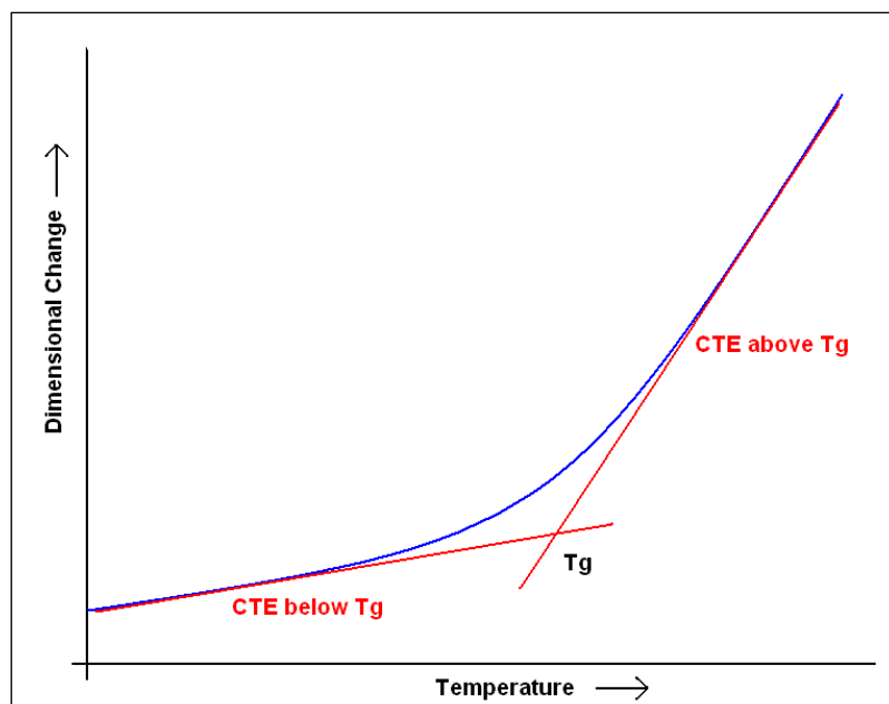
Figure 1 – Simple Tg curve showing CTE differences below and above the Tg
