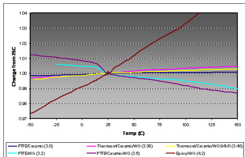
Figure 2 – TcDK (thermal coefficient of dielectric constant) curve of some common PCB laminate materials
