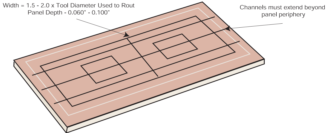
Figure 1 Pre-Rout Channels in Backer Board
