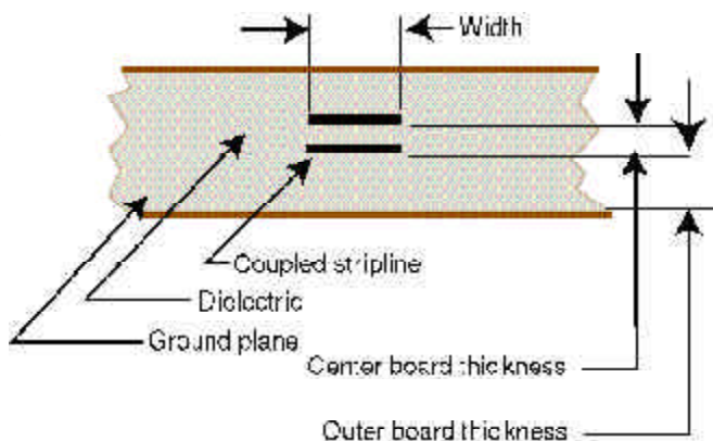
Figure 1: Cross sectional view of a typical broadside stripline coupler.
